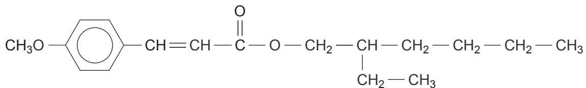
compound A
